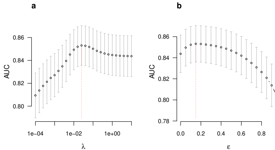
Figure 8: Cross-validation of transcription factor binding motif model using bbi with control sequences generated by 3 nucleotide mutations. Data set is from Khan et al. (2018) (sample ID MA0014.3; see text). (a) Pseudo-likelihood and (b) mean field inferences.
